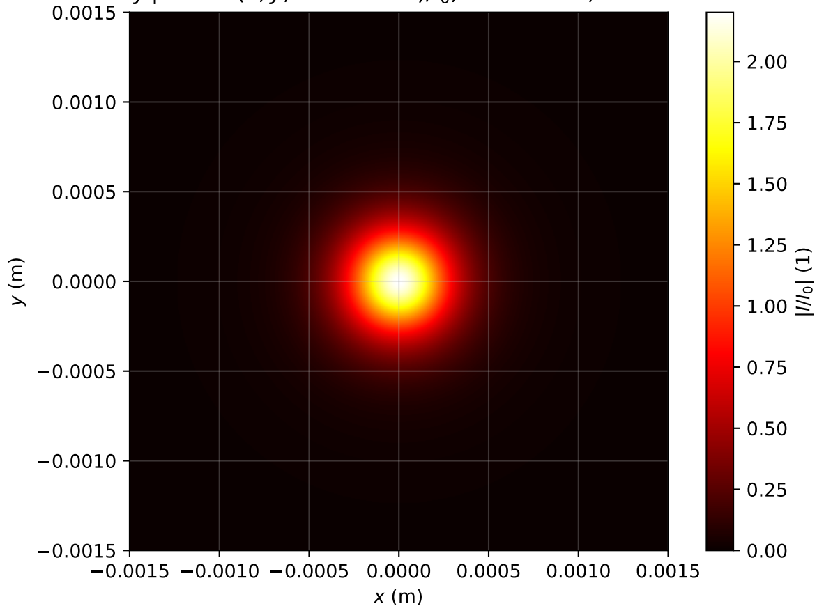
Intensity profile I(x, y, z = 2.149m)/I_0 , P_{in}=1.0P_{cr} , artificial time
